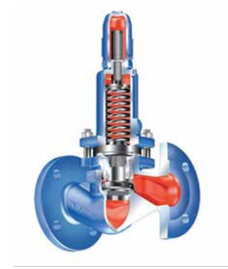
Pressure Regulating Valve
