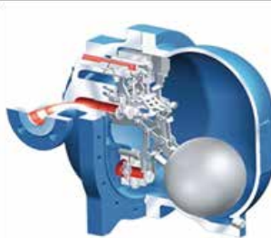
Ball Float Trap
