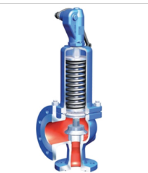
Safety Valve
